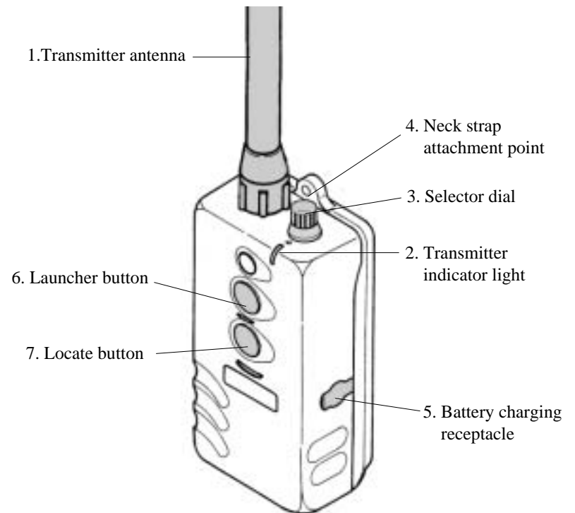
dogtra RRS transmitter
