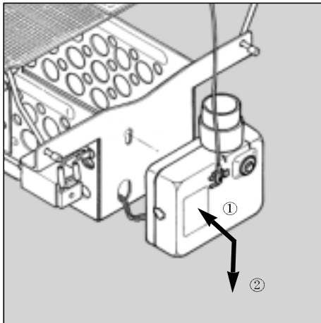
Figure 5. Mounting the receiver.
